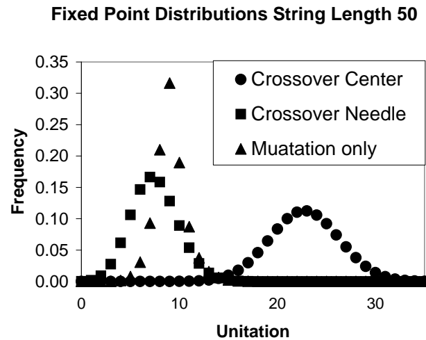
Figure 3: Fixed Point Distributions, \ell = 50 , k = 10 , a = 5 , b = 5 , \mu = 0.01
